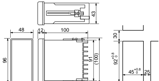
Panel cutout
