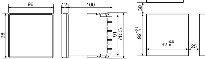
Panel cutout
