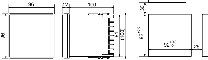
Panel cutout
