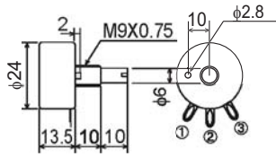
Volume (Resistance:5kΩ,B)
