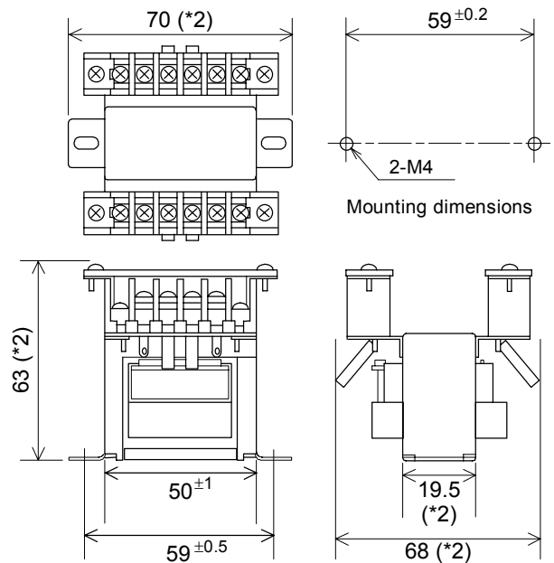
Fig. 2.3 Dimensions (Power feed transformer)
