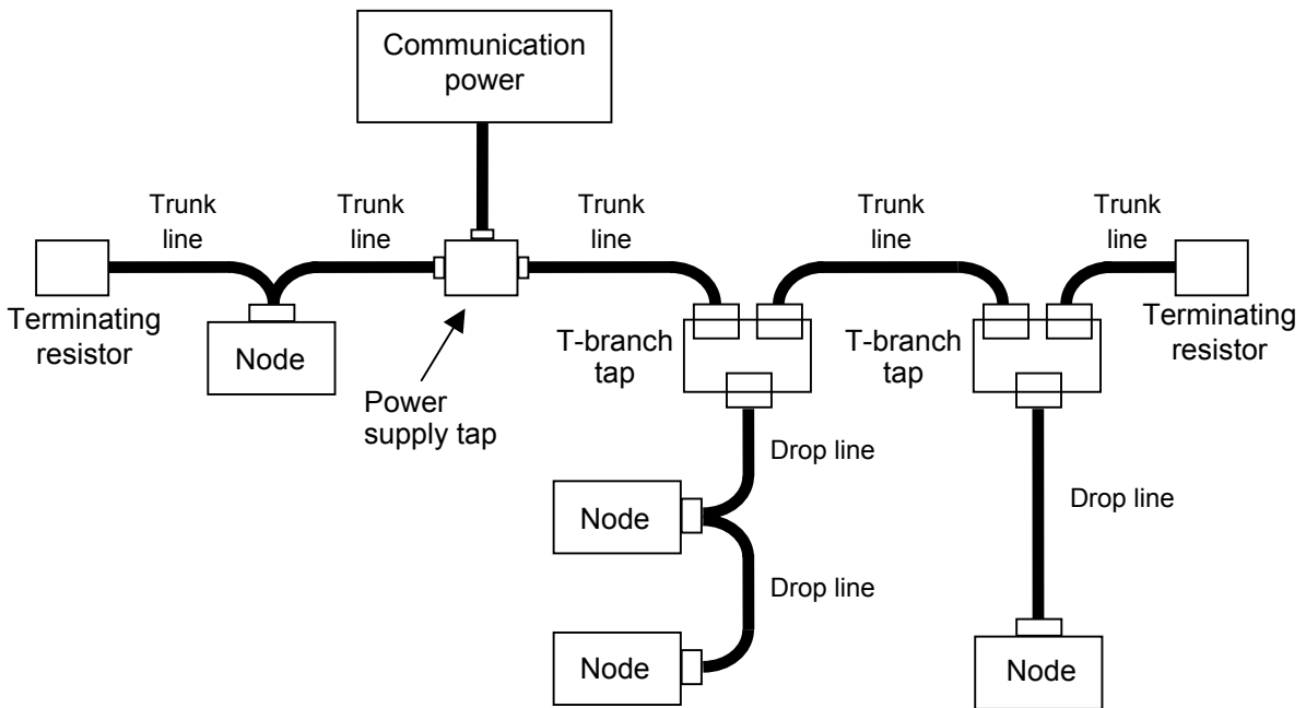
Network configuration example
