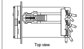
Fig. 7: Image of how to bend each solderless terminal lug
