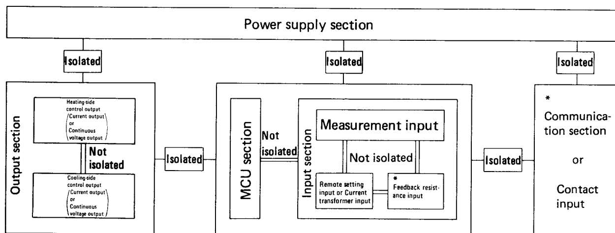
REX-F400 circuit configuration
