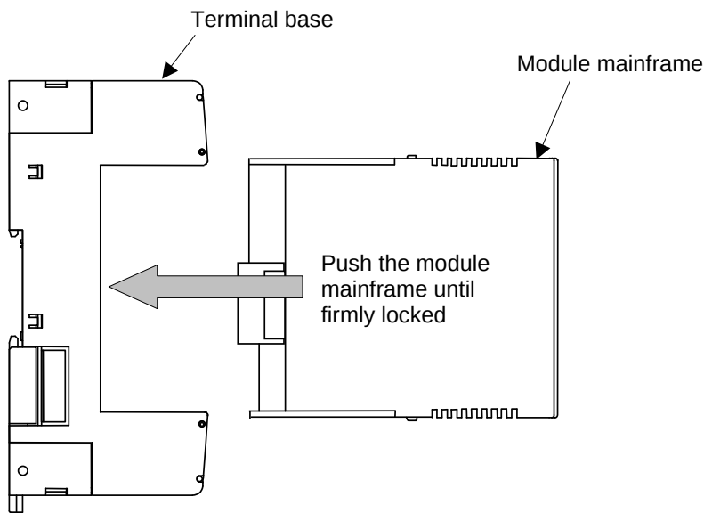
Mounting the module mainframe
