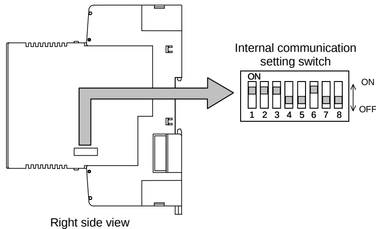
[Internal communication setting switch]
