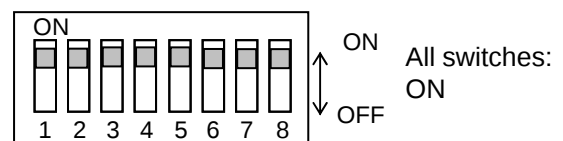
PLC communication setting switch
