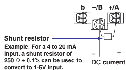
DC current input
