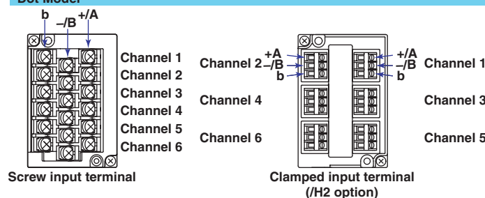
Channel location on the input terminals
