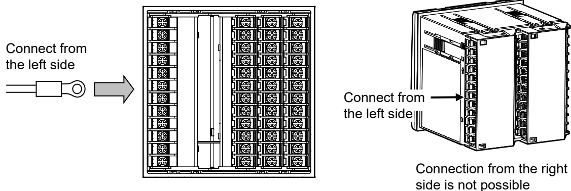
Fig. 3.2 Wiring direction
