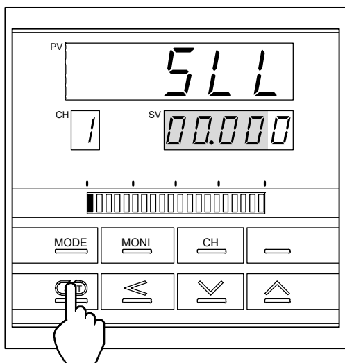
Setting limiter (low)
