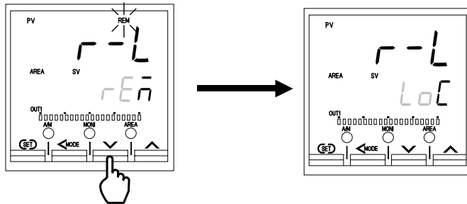
Remote/Local transfer
