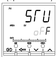
Startup tuning (ST) (Operation mode)
