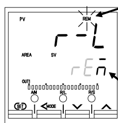
Operation mode Remote/Local transfer (Remote mode)
