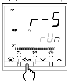
RUN/STOP transfer (Operation mode)
