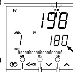
PV/SV monitor (Remote mode)
