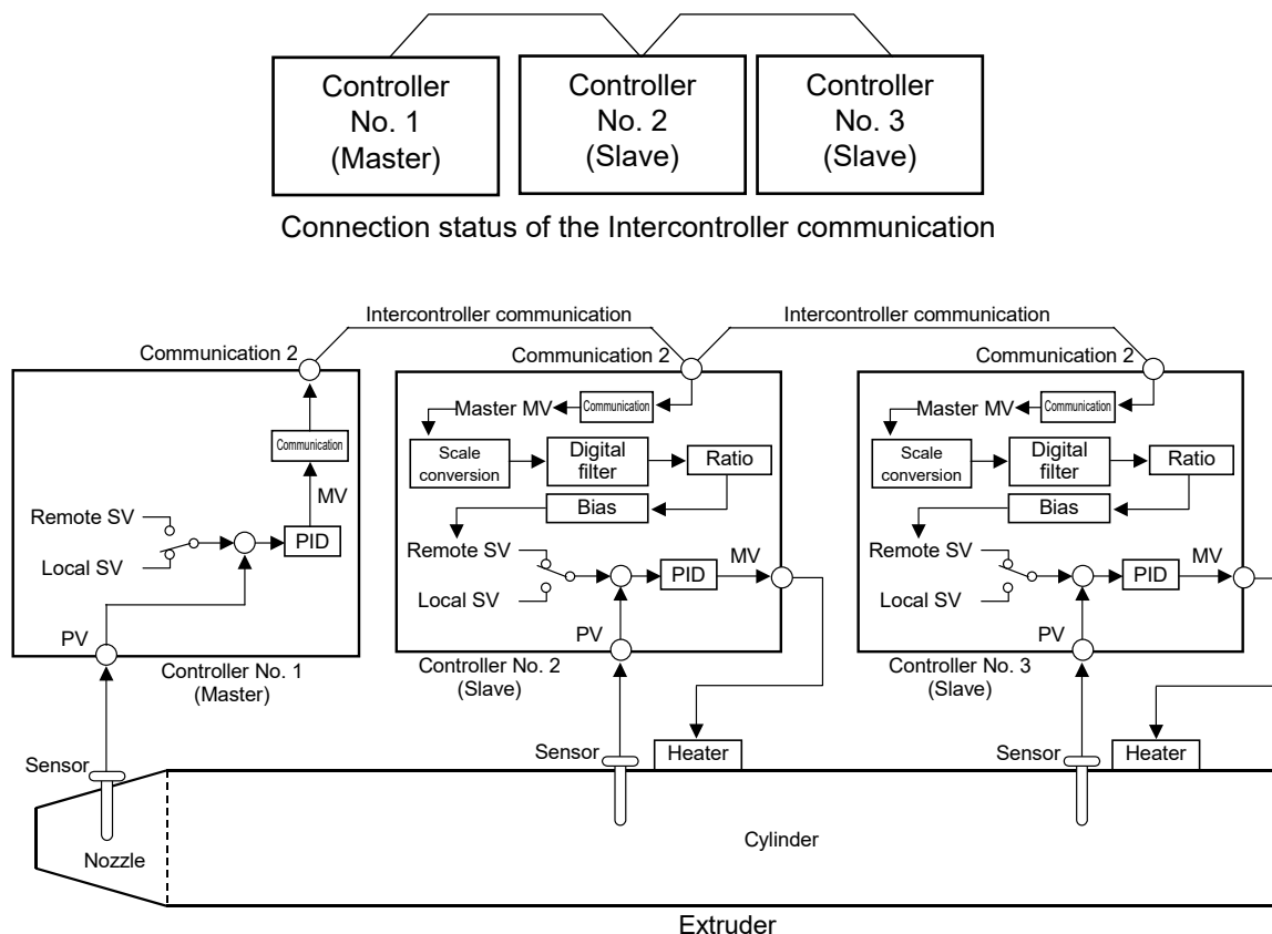
Block diagram of Cascade control by Intercontroller communication
