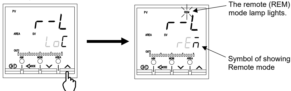
Remote/Local transfer
