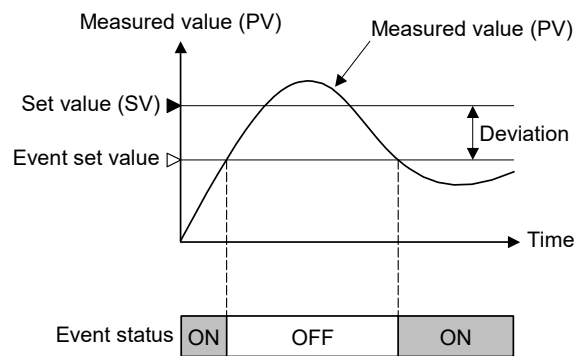
[Without hold action]
